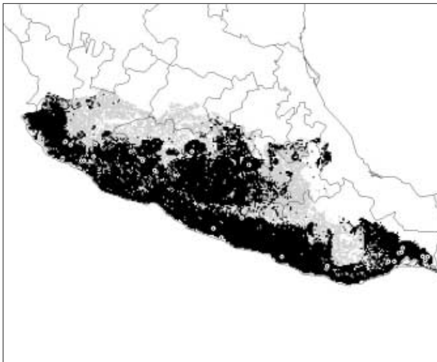
Figure 3. Projected effects of global climate change on the geographic distribution of the West Mexican Chachalaca Ortalis poliocephala : present distribution is shown in grey and black, and projected post-change distribution is in black; specimen-based distributional points are shown as dotted circles.
