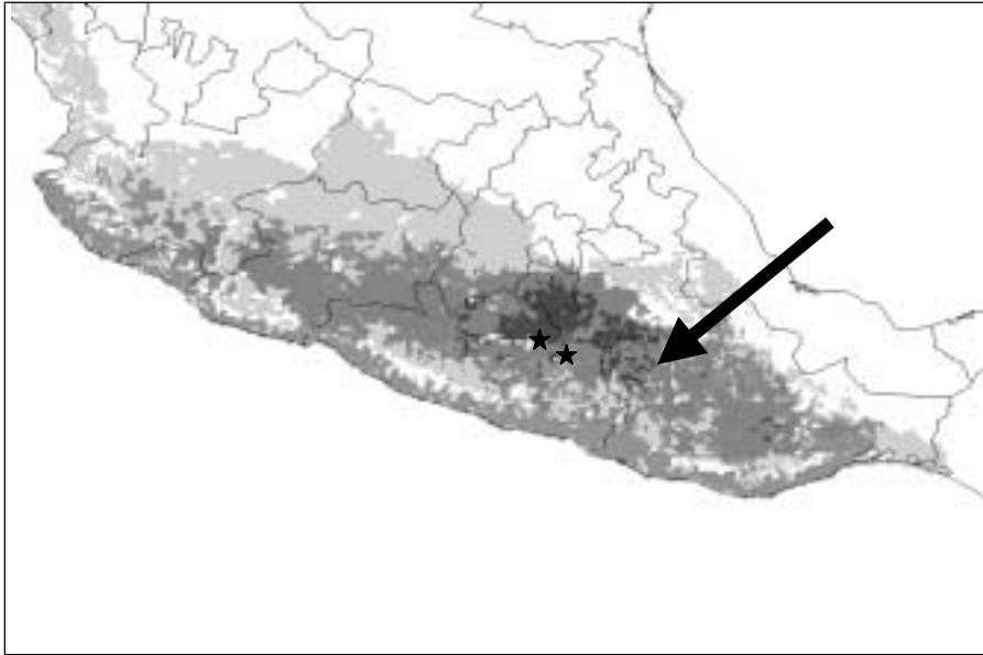
Figure 2. Richness of 16 species endemic to western Mexican tropical dry forests, showing increasing species richness as darker shades of grey. Locations of two biosphere reserves are shown with stars, coinciding with primary concentration of 12 species; the arrow indicates a secondary concentration, in which all four remaining species are represented.
