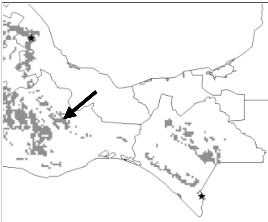
Figure 1. Distributional prediction (grey shading) for Slaty Finches Haplospiza rustica in Mexico based on two known specimen localities (black stars), showing third site discovered in 1995 (arrow).
